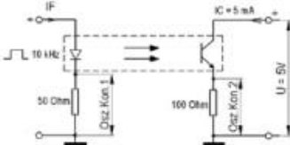
Test Circuit
